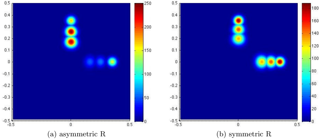
Figure 3: This figure illustrates that, except for particular symmetry conditions, a single Dirac mass is exhibited by Lotka-Volterra equations. We depict the density n with asymmetric (left) and symmetric (right) growth rate R plotted for t = 5, 90 and 180 in units of dt .
