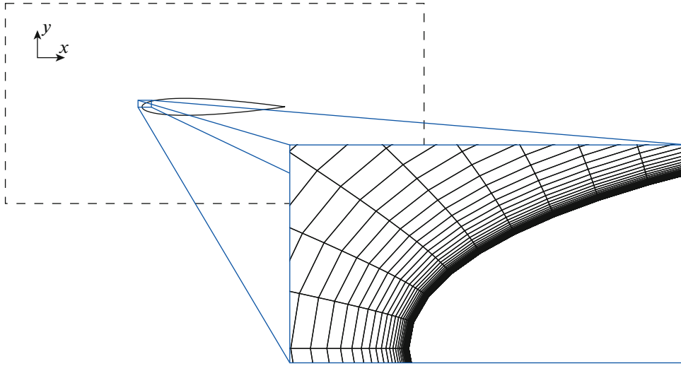
Fig. 5. Mesh configuration.
