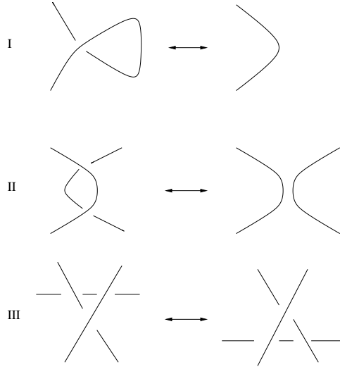
Figure 1: Reidemeister moves.
