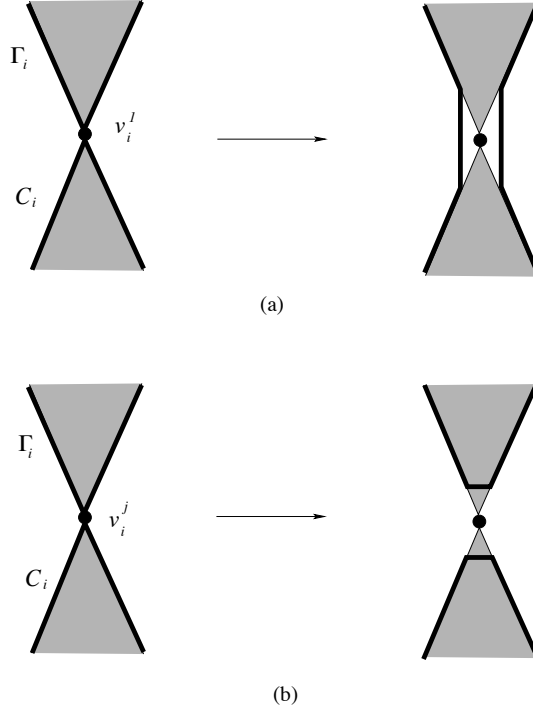
Figure 6: Modifications around a vertex for constructing \Gamma_h . vertices.
