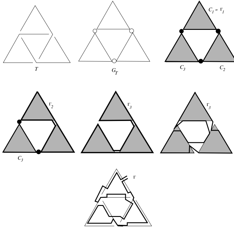
Figure 9: Construction of curve \Gamma for a Trefoil diagram.
