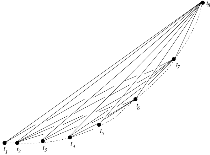
Figure 3: Projection of C(8) .
