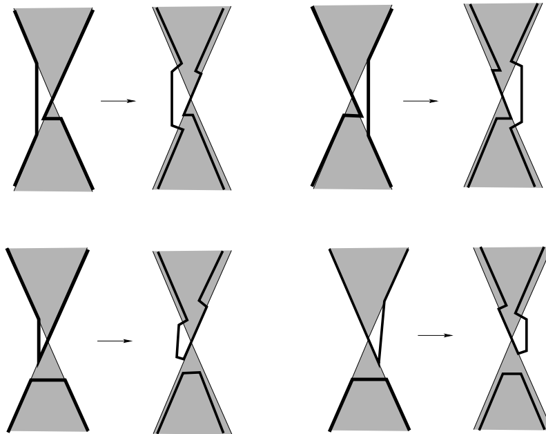
Figure 8: Moving \Gamma_h away from D(K) .
