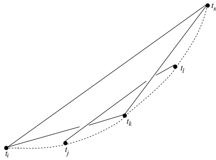
Figure 4: Edges with the crossing property.
