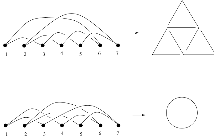
Figure 12: Non-reducible cycles for m = 7 .
