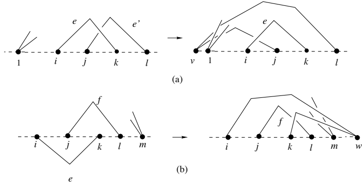
Figure 10: Fixing up upper and lower arcs.
