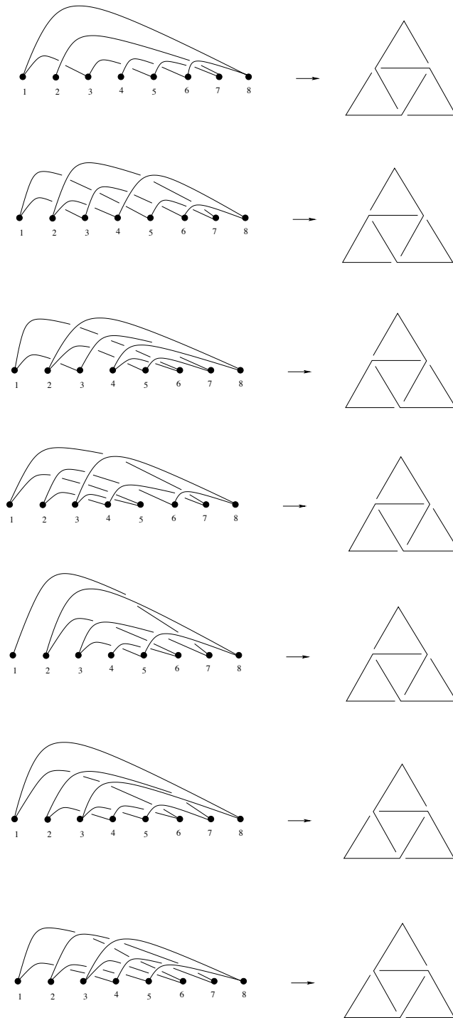
Figure 13: Non-reducible cycles for m = 8 .
