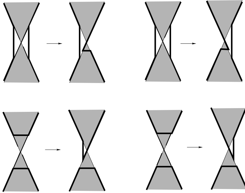
Figure 7: Local changes made to \Gamma_h .
