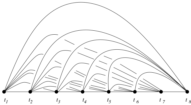
Figure 5: Representation of the diagram D(C(8)) .
