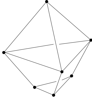
FIGURE 2. Configuration of 7 points without transversal line to the convex hull of the 4-sets.
