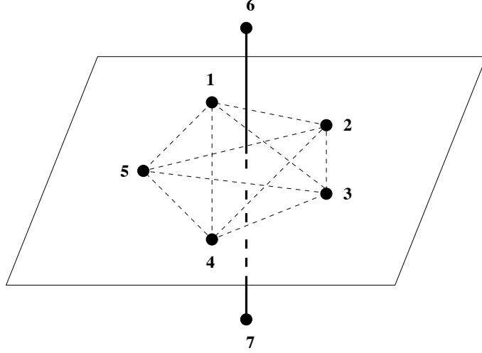
FIGURE 1. \overleftrightarrow{67} is a transversal line of all tetrahedrons.
