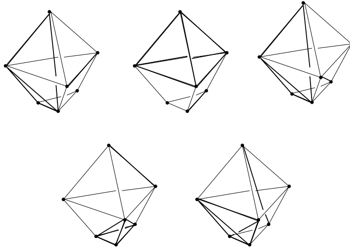
FIGURE 3. Transversals missing a tetrahedron.
