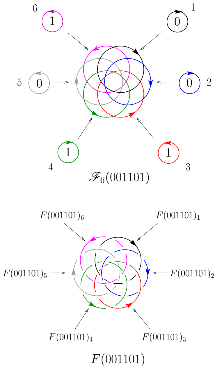
FIGURE 14. The oriented arrangement \mathcal{F}_6(001101) and its induced link, the flower link F(001101) . We indicate the six components of F(001101) .
