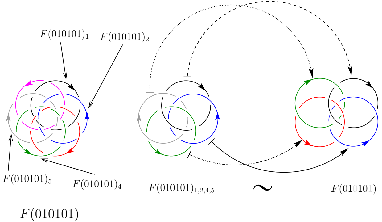
FIGURE 19. Illustration of Observation 38.
