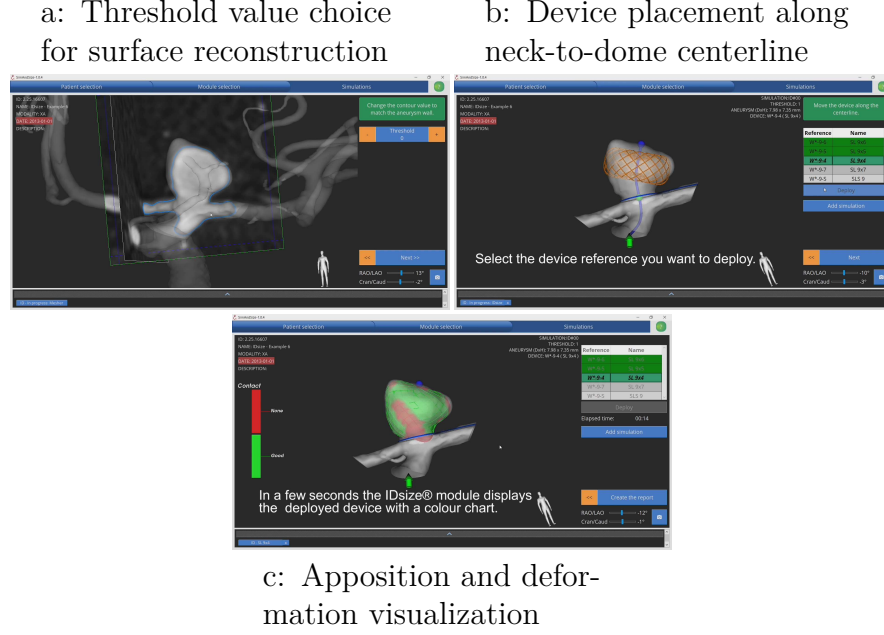
Figure 4.4: Sim&Size ® steps for WEB device deployment. Taken from https://sim-and-cure.com/ .
