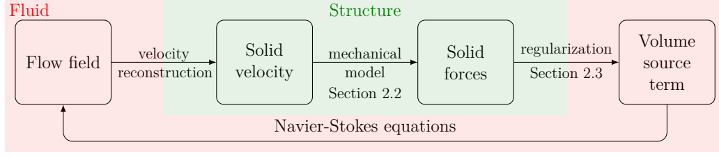
Figure 2.2: Main principles of the Immersed Boundary Method (IBM). Steps involving fluid and solid parts are highlighted in red and green, respectively. The sections involving the main developments are indicated for the ease of comprehension.
