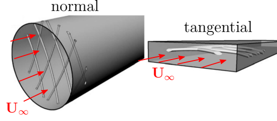
Figure 3.7: Augsburger normal (left) and tangential (right) configurations. Upstream velocity are represented in red at the inlet sections of each case. Taken and modified from [7]
