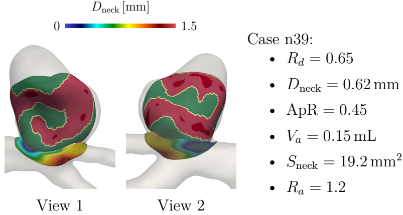
Figure 4.10: Case n39 example for distance to device D_{\text{neck}} and contact apposition ratio \text{ApR} maps. Red portions on the device surface are apposed to the aneurysm sac and summed for the computation of S_{\text{apposed}} in Table 4.3.
