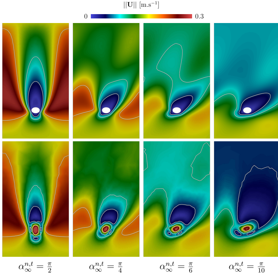
Figure 2.10: Velocity fields and contours for conformal (first line) and edge-based IBM (second line) approaches on a plane placed diagonally to the 3D domain for various \alpha_{\infty}^{n,t} angle of attack. The operating point is (\text{Re}, \tilde{W}/D, \alpha_{\infty}^{l,t}) = (5, 8, 0) . A good qualitative agreement is reached by the current model when being compared to conformal velocity fields.
